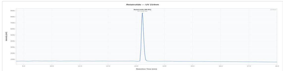
Retatrutide 10mg - 0326-A: UV Chromatogram
