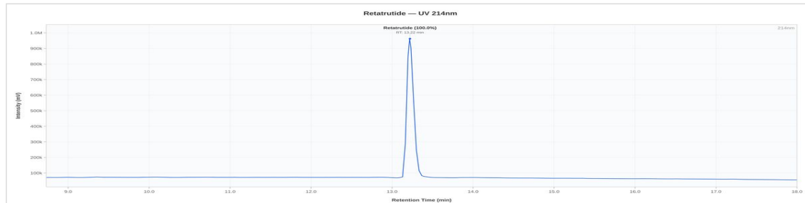
Retatrutide 60mg - 0326-A: UV Chromatogram
