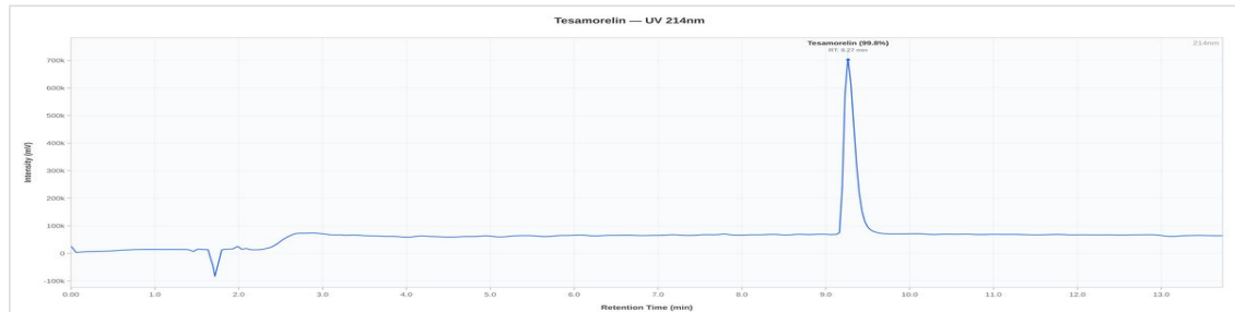
Tesamorelin 20mg - 0326-U: UV Chromatogram
